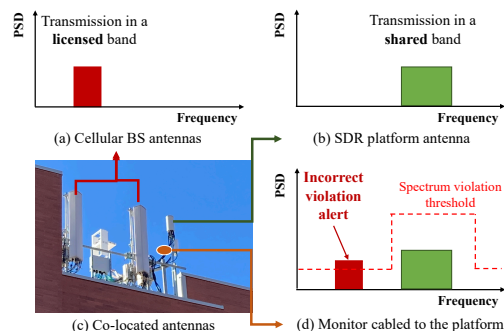
Fig. 1: A co-located base station’s signal is incident to an SDR platform’s antenna. If the monitor cannot separate the two signals, it may believe that its own SDR’s transmitted signal is violating spectrum rules, which would be a false alarm.
