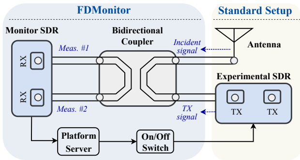
Fig. 2: Architecture and the closed-loop control of FDMonitor, and the standard setup of its monitored SDR platform.
