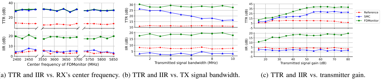
Fig. 7: TTR(transmit signal separation) and IIR(incident signal separation) comparisons between FDMonitor and SMC. (a) Receiver’s center frequency : both methods present similar TTR increase, but FDMonitor results in superior IIR. (b) Transmitted signal bandwidth : FDMonitor is consistent across bandwidths whereas SMC degrades as bandwidth increases. (c) Transmitter gain : FDMonitor improves both while SMC reduces IIR with the increasing gain.
